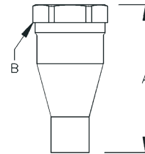
Female Innengewinde
