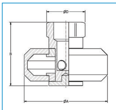
HWD Dimensions (mm)
