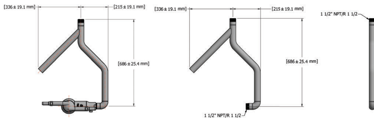
Adapter with HydroWhirl Orbitor 2 x 10
