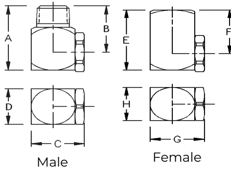
Hollow Cone 80° (XPN)
