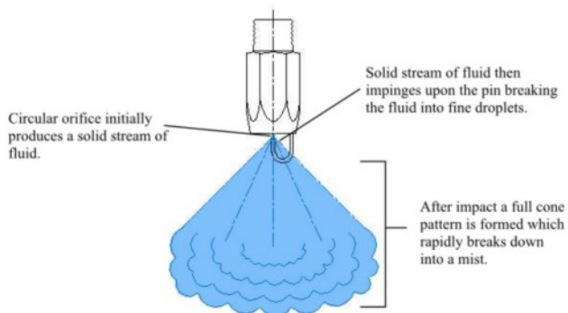
Impingement misting nozzle
